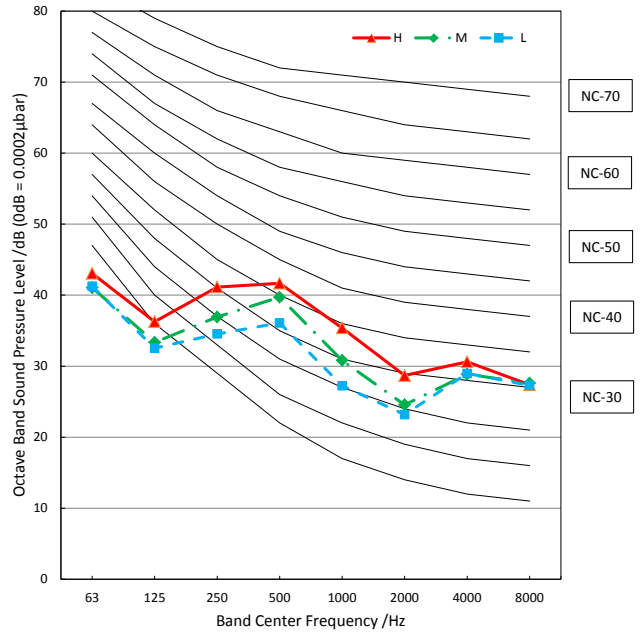
MCD1-24HRFN1-MT0W(GA)
