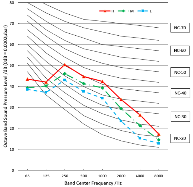
MCD1-24HRFN1-MT0W(GA)
